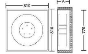
Recessed Mounted
