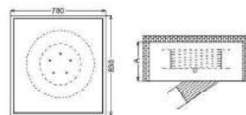
Recessed Mounted
