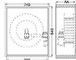
Recessed Mounted
